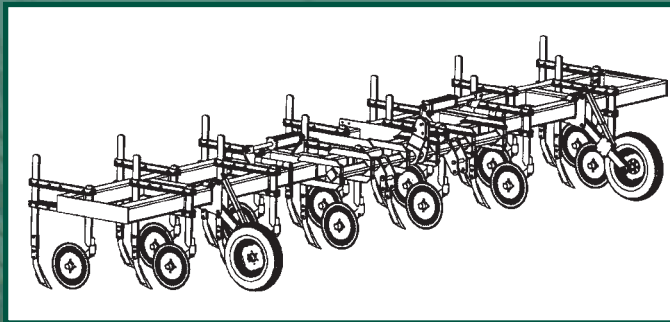
1 x 2 APPLICATOR
